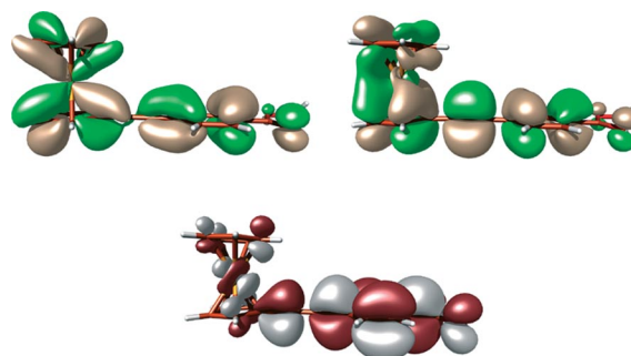
Figure 4. Orbitals 79 (top left), 86 (top right) and 90 (bottom) of 3e (all at the 2% probability level). The two partially bonding/antibonding 79 and 86 and the completely antibonding 90 are partners to orbital 77; orbital 90 is the LUMO.
