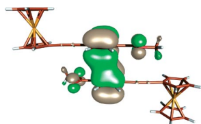
Figure 5. Orbital 161 of the 3e ... 3e dimer (2% probability level).
